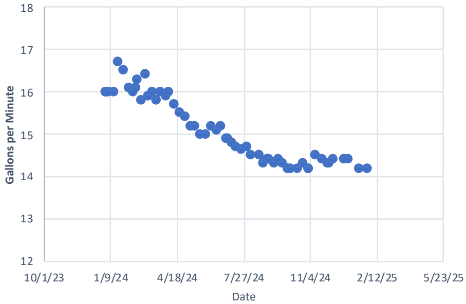
Flow Rate From Spring
